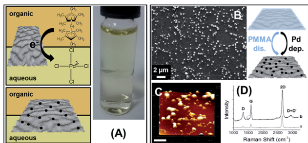
Fig. 3 (A) Schematics of the \text{PdCl}_4^{2-} reduction by DecMFC via CVD GR at the interface (above) by forming the black dots marked Pd NPs (below), shown on the photograph, and the Raman spectra (D, 633 nm) of the pristine and Pd-deposited CVD GR. SEM (B) and AFM (C, scale bar: 1 \mu\text{m} ) images and schematics of the Pd NPs decorated CVD GR layer, when the metal deposition and the dissolution of the PMMA takes place simultaneously. The interfacial contact time of deposition was 1 min in the all cases. The DCE/5-nonanone ratio was 1 : 4.
