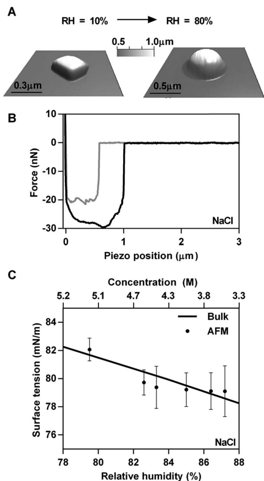
Fig. 2 Experimental results of AFM based surface tension measurements of a ~500 nm NaCl droplet. (A) 3D image of a solid NaCl crystal at 10% RH and deliquesced NaCl particle at 80% RH. (B) Experimental force plot on a NaCl droplet. The approach data is in grey and the retract data is in black. (C) Surface tension measurements (average and standard deviation) as a function of RH (bottom axis) and solute concentration (top axis). Predicted data is obtained from bulk solution surface tension measurements and is shown as the solid line.
