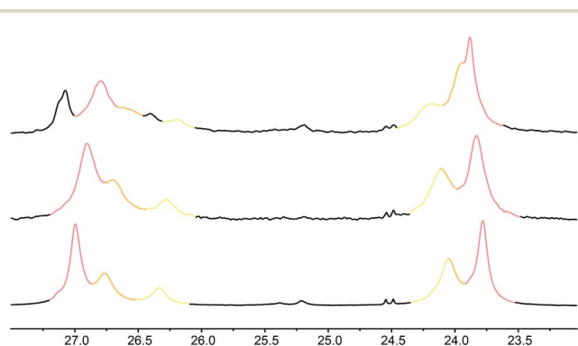
Fig. 7 Illustrative ^{13}\text{C} NMR spectra of 7a (top), 7b (middle) and 7c (bottom) in 9 : 1 methanol : chloroform, with peaks arising from the 100%, 50% and 25% labels indicated by colours used in Fig. 6.
