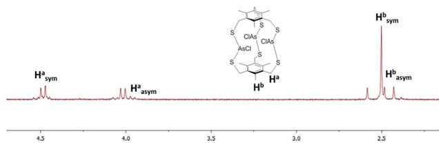
Fig. 4 ^1\text{H} NMR spectrum for \text{As}_3\text{L}^{\text{Me}}_2\text{Cl}_3 macrobicyclic. The signals from the symmetric and asymmetric macrobicyclic are labeled.
