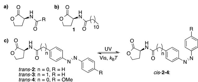
Fig. 1 Molecular structures of AHLs. (a) The structure of naturally-occurring AHLs, where R is usually an alkyl chain varying in length between 4 and 18 carbon atoms. (b) Structure of a naturally occurring auto-inducer ( 1 ) (c) Three photoswitchable analogs ( 2 , 3 and 4 ) that can undergo trans–cis photoisomerization upon UV-light irradiation and cis–trans isomerization upon visible-light irradiation and thermal relaxation.
