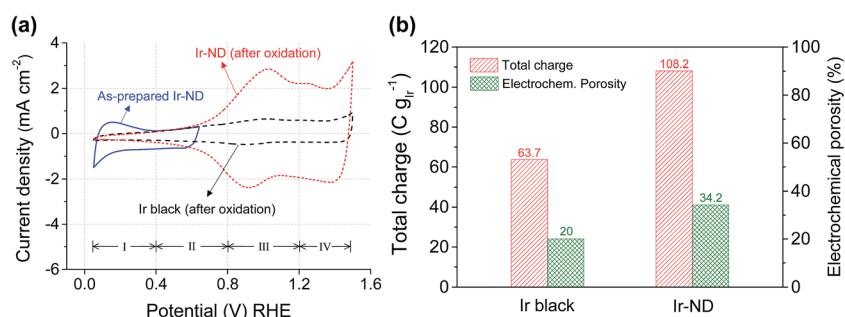
Fig. 3 Surface redox electrochemistry of commercial iridium black and iridium nanodendrites (Ir-ND): (a) cyclic voltammograms (CVs) of as-prepared and oxidized nanodendrites. Conditions: 25 C, N 2 -purged 0.05 M H 2 SO 4 , 20 mV s -1 . The CV of the as-prepared Ir nanodendrites (Ir-ND) was recorded between +0.05 to +0.64 V RHE to avoid Ir oxide formation. (b) Electrochemical total charge and porosity of Ir-ND and Ir black.
