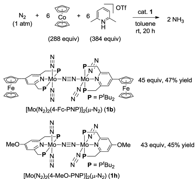
Scheme 3 Catalytic formation of ammonia from molecular dinitrogen in the presence of 1b and 1h as catalysts by using larger amounts of cobaltocenium and proton source.
