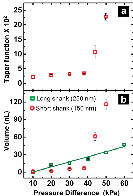
Fig. 2 (a) Variation in taper function with pressure for \sim 150 nm short shank pipettes. (b) Volume of sample aspirated as a function of pressure difference for long ( \square ) and short ( \circ ) shank pipettes. For all plots, n = 3 .
