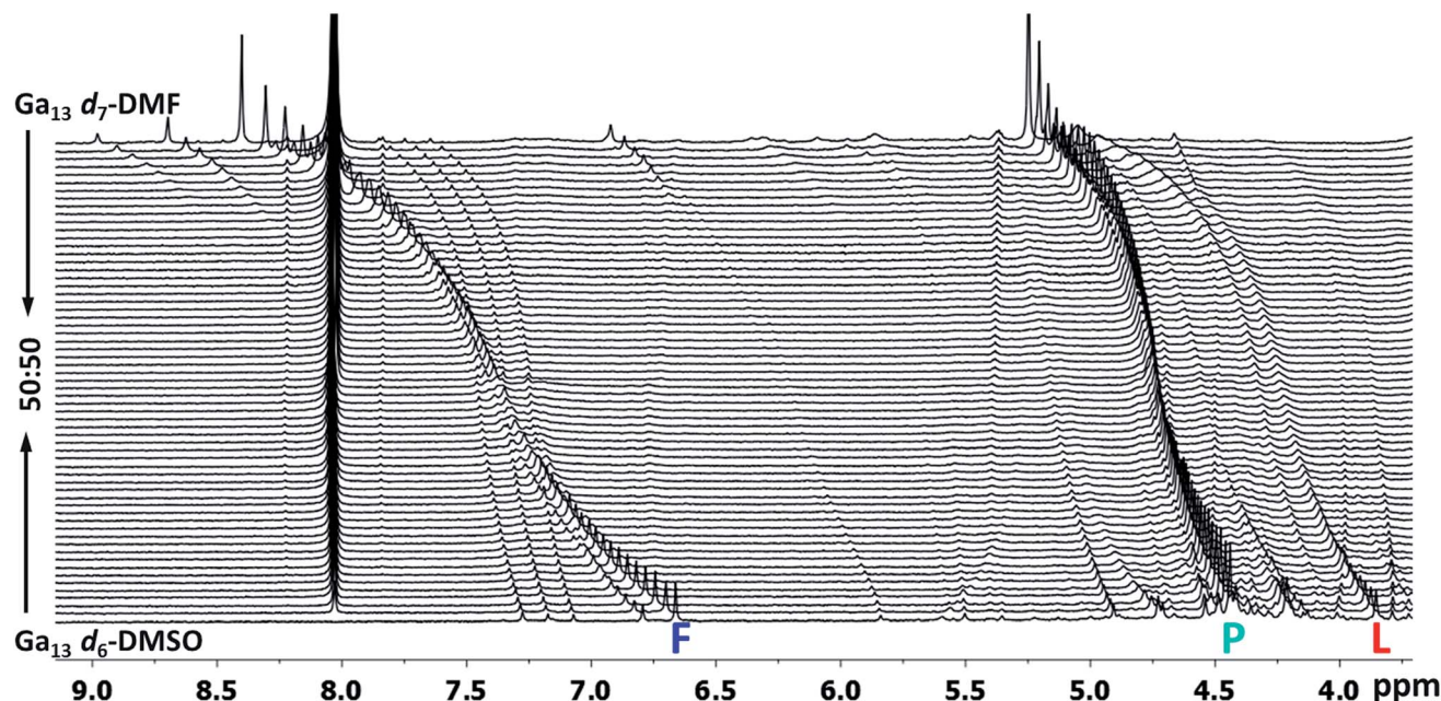
Fig. 16 Stacked titration data indicating that only the H_{GaGaGa}^{\mu_3} (F), H_{GaGaGa}^{\mu_{2int}} (L), and H_{GaGaGa}^{\mu_{2ext}} (P) protons translate from the 100% d_6 -DMSO to the 100% d_7 -DMF spectrum. The triplet that persists in the 7.0 to 7.5 ppm region is attributed to ammonia in the sample. 77
