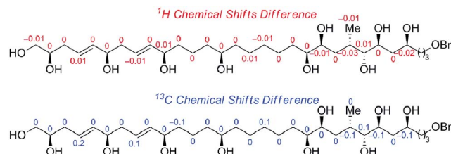
Fig. 3 Comparison of ^1\text{H} and ^{13}\text{C} NMR data of synthetic and natural polyol fragment of AM3.
