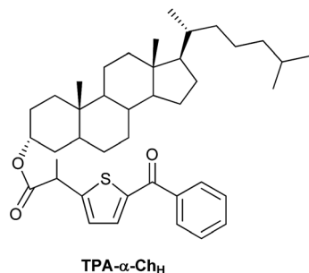
Chart 2 Chemical structure of the TPA derivative of hydrogenated cholesterol.
