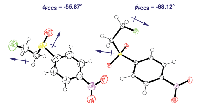
Scheme 2 Syntheses and X-ray crystal structure analyses 14 of linear sulfoxide 6 and sulfone 7 . (a) m CPBA (1.0 eq.), CH 2 Cl 2 , 0 °C to rt, 26 h; (b) m CPBA (3.0 eq.), CH 2 Cl 2 , 0 °C to rt, 17 h. Thermal ellipsoids shown at 50% probability level.
