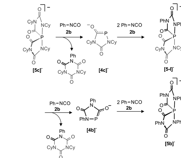
Scheme 3 \text{P}^- transfer from [5\text{c}]^- to [5\text{b}]^- . The heterocycles [4\text{c}]^- and [4\text{b}]^- as well as the spiro-anion [5\text{-I}]^- were not observed under the reaction conditions but are likely intermediates.
