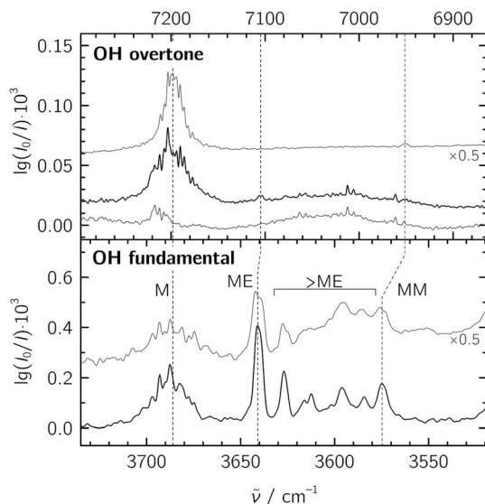
Fig. 2 Jet-FTIR spectra of methanol : ethene mixtures in the fundamental (bottom) and overtone (top) regions. Bottom panel: mixtures with M : E ratios of \sim 1 : 20 (black trace, with approximate number densities of 3 \times 10^{13} \text{ cm}^{-3} for M, 7 \times 10^{11} \text{ cm}^{-3} for ME and 3 \times 10^{12} \text{ cm}^{-3} for ME based on anharmonic B2PLYP-D3BJ/VTZ IR intensities) and \sim 1 : 7 (grey trace, intensity-scaled by 0.5) expanded at a stagnation pressure of P_s = 0.75 bar. ">ME" indicates signals from larger clusters which we do not interpret explicitly. Top panel: overtone spectra of the \sim 1 : 7 M : E mixture (strong black trace), E (thin black trace) and M (grey trace, from ref. 20, intensity-scaled by 0.5). The wavenumber scale in the top panel is compressed by a factor of 2 and shifted to match the M monomer band centers in order to visualize the change in diagonal anharmonicity in the ME and MM structures.
