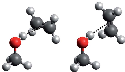
Fig. 1 “Perpendicular” (left) and “parallel” (right) ME structures. Only the former is predicted to be a stable minimum, but low barriers to the torsion of the ethene unit may leave artifacts in harmonic and anharmonic approaches.
