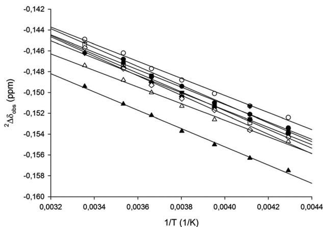
Fig. 3 The similar temperature dependence of the two-bond isotope effect ( {}^2\Delta_{\text{obs}} ) measured on C-3 of 1-I to 9-I indicates that the [\text{N}-\text{I}-\text{N}]^+ halogen bond is static and symmetric in solution, regardless of the counterion. \circ \text{BF}_4^- , \blacktriangledown \text{ClO}_4^- , \blacksquare \text{PF}_6^- , \square \text{SbF}_6^- , \bullet \text{TfO}^- , \blacklozenge \text{TsO}^- , \triangle \text{NO}_3^- , \blacktriangle \text{CF}_3\text{CO}_2^- , and \diamond \text{BF}_4^- .
