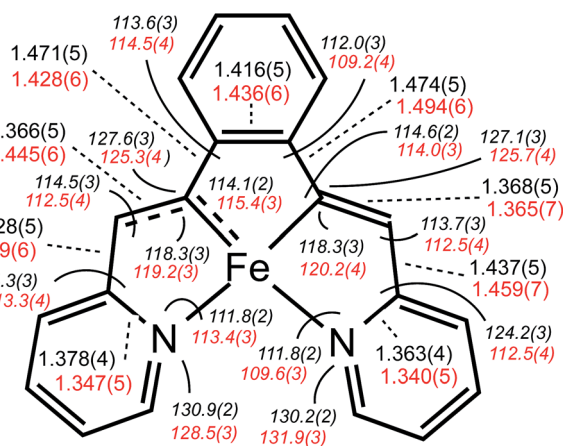
Fig. 3 Comparative ligand metric parameters (distances ( \text{\AA} ), dashed black lines; angles ( ^\circ ), italics ), curved black lines) for Fe(II) (\text{bdvp})\text{Fe}(\text{PMe}_3)_2 ( 1-PMe}_3 , black) vs. Fe(IV) [(\text{bavp})\text{Fe}(\text{PMe}_3)_2][\text{BAR}^{\text{F}}_4] ( 4-PMe}_3 , red).
