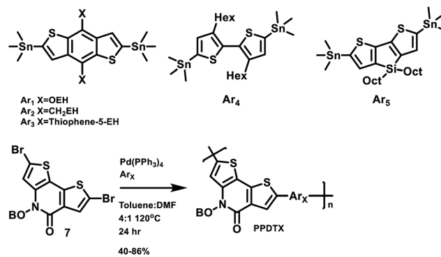
Scheme 2 Synthetic route to PPDT series polymers.
