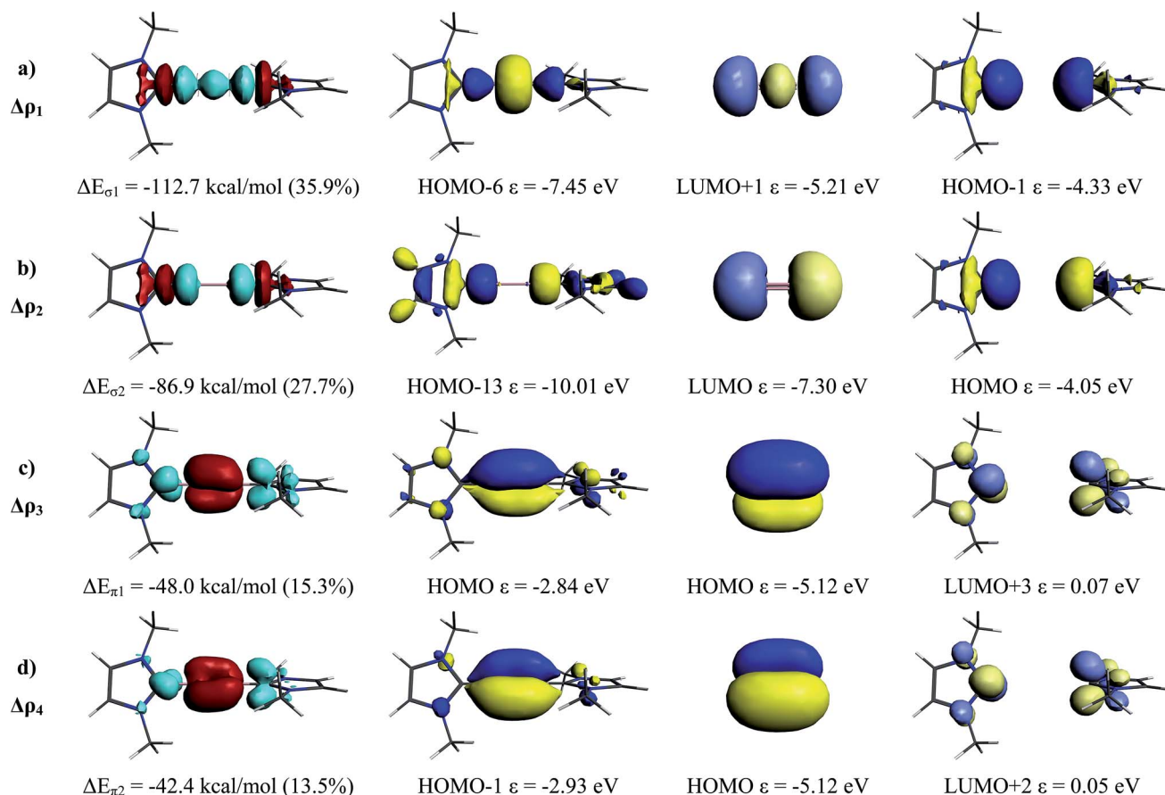
Fig. 3 Plot of the interacting donor and acceptor orbitals and calculated eigenvalues \epsilon of (NHC^{Me})_2 and (\Sigma_g^+) B_2 (right two columns) and matching MOs of the complex NHC^{Me} \rightarrow B \equiv B \leftarrow NHC^{Me} (second column from the left). Plot of the deformation densities \Delta\rho with connected stabilization energies \Delta E of the four most important orbital interactions in B_2(NHC^{Me})_2 which indicate the associated charge flow red \rightarrow blue.
