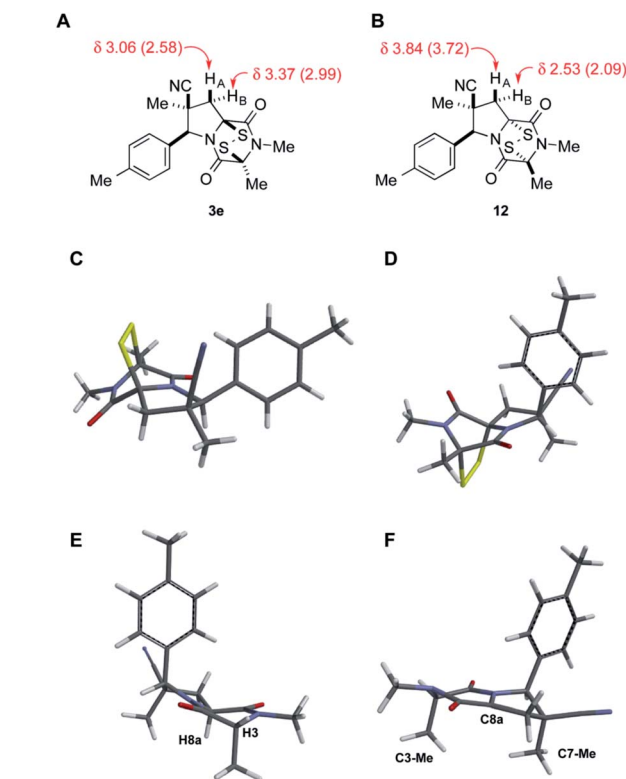
Fig. 3 Representative data used to assign the relative configuration of the disulfide bridge in ETP products, X-ray model of dioxopiperazine 8e , and a computation model of the derived angular enolate. (A and B) show the observed (in CDCl 3 ) and calculated (in parentheses) chemical signals of the methylene hydrogens of the pyrrolidine ring of ETP diastereomers 3e and 12 . (C) is the X-ray model of 3e . (D) is the computational model (B3LYP/631-G*) of 12 . (E) is the X-ray model of dioxopiperazine 8e . (F) is the predominant conformer (B3LYP/631-G*) of the angular enolate formed from dioxopiperazine 8e .
