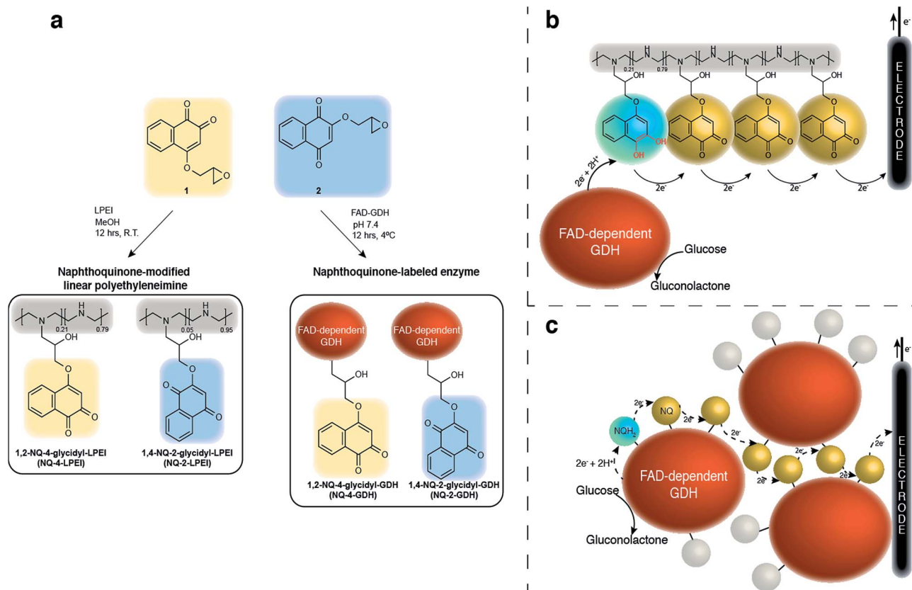
Fig. 1 The rational design of naphthoquinone (NQ) derivatives allows for desirable covalent immobilization of two methods. Mediated bioelectrocatalytic glucose oxidation can subsequently occur by flavin adenine dinucleotide-dependent glucose dehydrogenase (GDH). (a) NQ derivatives were designed and synthesized to have epoxide functionalities, allowing their covalent attachment to a linear polyethylenimine backbone (forming a NQ redox hydrogel, NQ-LPEI) and direct labeling of GDH. (b) NQs are able to undergo self-exchange whereby electrons and protons diffuse along a functionalized polymer backbone to an electrode surface. (c) Epoxide functionalities permit multipoint covalent NQ attachment to GDH.
