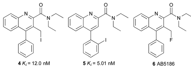
Fig. 2 Quinoline-2-carboxamides 4 , 5 and 6 .
