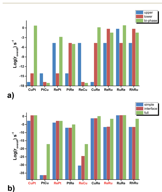
Fig. 3 Activity ( \log(r_{\text{overall}}) ) comparisons of nine bi-phase surfaces among (a) those from the upper phase, lower phase and bi-phase surfaces, respectively, (b) the simple, interface and full kinetic models, where the reactive-noble bi-phase surfaces are highlighted in red.
