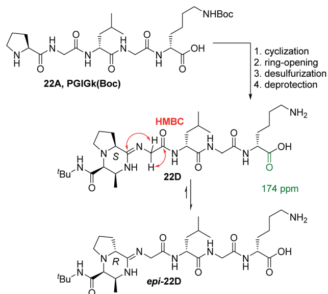
Scheme 4 Formation of amidine peptide products along with \text{P}_{\text{Hz}\alpha} epimerization.
