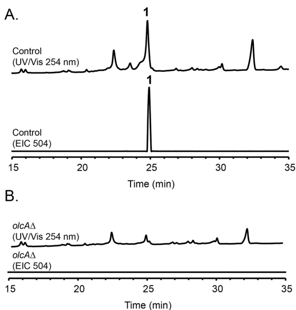
Fig. 2 HPLC profiles of extracts from (A) parental strain and (B) olcΔΔ strain as detected by UV-vis at 254 nm and mass spectrometry in positive mode of extracted ion chromatogram (EIC) at m/z = 504 .
