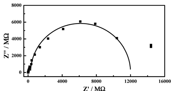
Fig. 4 The electrochemical impedance spectroscopy of the redox couple of \text{Co}(\text{CN})_6^{3-/4-} in the NaCl microcrystals. The initial concentration of \text{Co}(\text{CN})_6^{3-} for the crystal culture is 10 mM.
