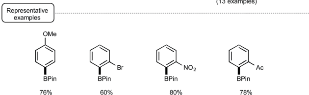
Scheme 31 Visible-light-induced borylation of aryldiazonium salts.
