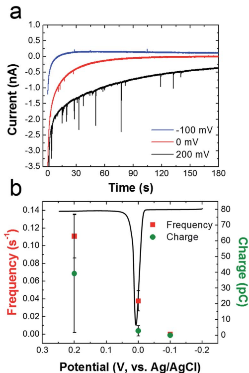
Fig. 7 (a) i – t curves obtained for cMμB–DNA–AgNP conjugate collisions in the presence of a magnetic field. The concentration of cMμB–DNA–AgNP was 100 aM, and the potentials applied to the Ni/Au UME for each experiment are indicated in the legend. (b) Plot of frequency and charge vs. the applied potential. The black curve is a representative Ag stripping voltammogram obtained for AgNPs dropcast onto a Au macroelectrode (2 mm). The scan started at -0.2 V and ended at 0.3 V. The scan rate was 50 mV s ^{-1} and the electrolyte was 100 mM PBCl buffer. The error bars were determined from three independent experiments at each potential.
