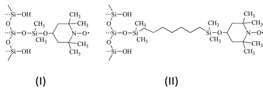
Fig. 3 Immobilized nitroxide material I (left) and II (right) used in SLIT ^1\text{H} DNP in normal liquids and \text{SF CO}_2 .
