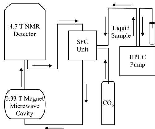
Fig. 4 Schematic drawing of apparatus for continuous-flow HPLC-DNP-NMR coupled with \text{SF CO}_2 (adapted from ref. 43, with the original figure shown in ESI†).
