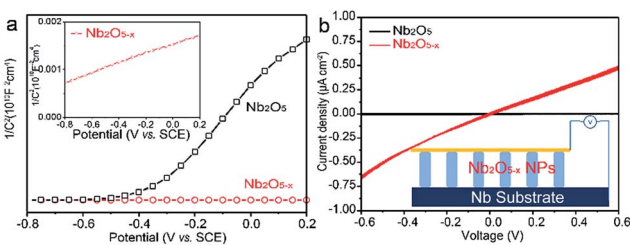
Fig. 3 (a) Mott-Schottky plots of \text{Nb}_2\text{O}_5 and \text{Nb}_2\text{O}_{5-x} NPs films at a frequency of 1\ \text{kHz} in the dark; (b) comparison of I - V curves of the samples; the inset is the schematic of the measurement.
