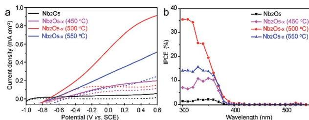
Fig. 4 (a) I - V curves measured under 100\ \text{mW}\ \text{cm}^{-2} simulated solar light generated by a 100\ \text{W} xenon lamp coupled with an AM 1.5G filter in 1\ \text{M} NaOH electrolyte; (b) IPCE spectra measured at 0.2\ \text{V} vs. SCE in 1\ \text{M} NaOH electrolyte.
