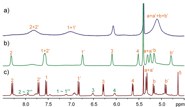
Fig. 5 Partial ^1\text{H} NMR spectra ( \text{CD}_2\text{Cl}_2 : \text{CD}_3\text{CN} = 1 : 1 , 2.0 mM) of an equimolar mixture of TA4 and \text{MeV}^{2+} at (a) 25 ^\circ\text{C} (400 MHz) or (b) -20 ^\circ\text{C} (600 MHz) and (c) TA4 and \text{AVA}^{2+} (400 MHz, 25 ^\circ\text{C} ).
