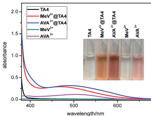
Fig. 6 UV-vis absorption spectra (1.0 mM, 25 ^\circ\text{C} ) of TA4, \text{MeV}^{2+}-2\text{PF}_6 , \text{AVA}^{2+}-2\text{PF}_6 , \text{MeV}^{2+}@\text{TA4} and \text{AVA}^{2+}@\text{TA4} . Inset: photos of the above solutions.
