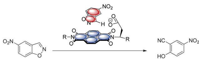
Fig. 37 Schematic representation of the anion– \pi supported Kemp's elimination as reported by Zhao et al. 11a,c
