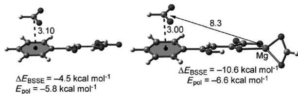
Fig. 44 Molecular structures of the formate complexes with PKDA and interaction energies ( \Delta E_{\text{BSE}} ) and the polarization contributions as calculated by Bauzá et al. (distances given in Å). Reproduced and adapted with permissions from John Wiley and Sons. 52b
