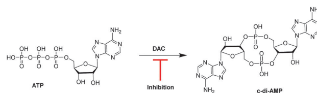
Fig. 1 Schematic of the synthesis of c-di-AMP by DisA from ATP. A DAC inhibitor will hinder the synthesis of c-di-AMP. 15
