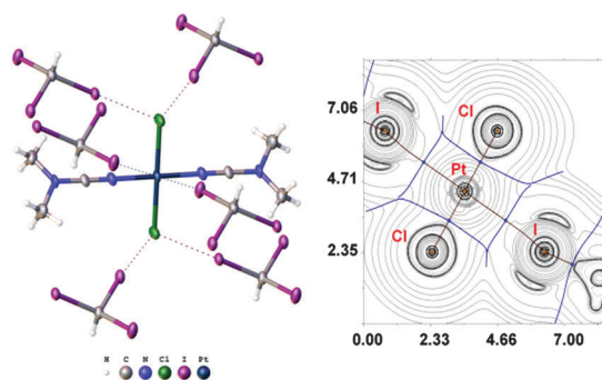
Fig. 1 Left: View of fragment \mathbf{1a} \cdot (\text{CHI}_3)_6 from \mathbf{1a} \cdot \frac{1}{2}\text{CHI}_3 \cdot \frac{1}{2}\text{CHI}_3 . Thermal ellipsoids are shown with 50% probability and short contacts are indicated by dotted lines. Coordinates of this fragment were applied in further DFT calculations. Right: Contour line diagram of the Laplacian distribution \nabla^2\rho(r) (cross-section along the plane \text{Pt–Cl–I} ) was received as a result of the topological analysis of the electron density distribution in the model structure. Bond paths are shown as brown lines, selected zero-flux surfaces – as blue lines, bond critical points (3, –1) are shown in blue, nuclear critical points (3, –3) – in pale brown, length unit – Å.
