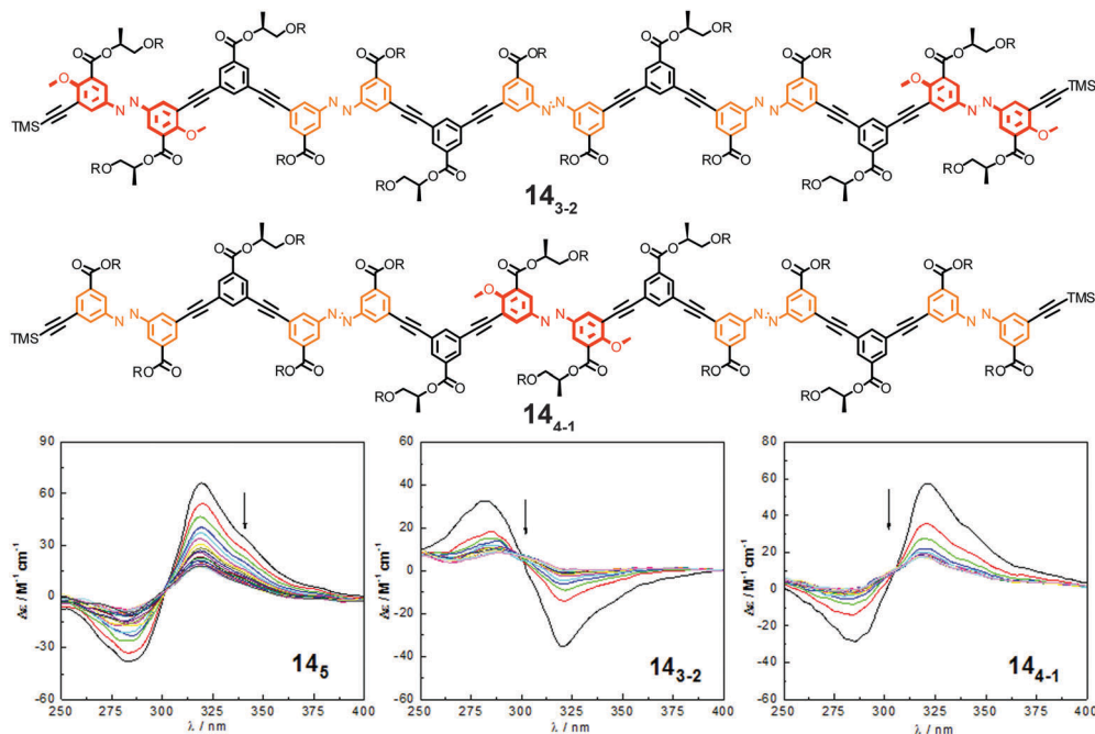
Fig. 18 Photoswitchable heterogeneous oligoazobenzene tetradecamers 14 3-2 and 14 4-1 (R = -(CH 2 CH 2 O) 3 CH 3 ) and the corresponding CD spectra ( 14 5 shown for comparison) during the course of irradiation at \lambda_{irr} = 358 nm in CH 3 CN at 25 °C. 108
