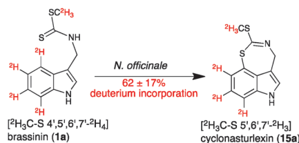
Scheme 4 Transformation of [\text{H}_3\text{C}-\text{S } 4',5',6',7'-\text{H}_4] brassinin ( 1a ) to cyclonasturlexin ( 15a ) in elicited leaves of watercress (percentage of deuterium incorporated shown in Table 2).
