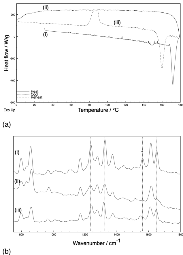
Fig. 1 (a) DSC thermograms and (b) Raman spectra recorded at (i) 30 °C before heating [form I], (ii) 30 °C after quench cooling [amorphous] and (iii) 110 °C [form III] after reheating for a 10% lactose containing sample of paracetamol (annotated with key spectral shifts observed from I to III).
