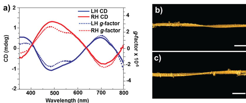
Fig. 5 (a) CD (solid line) and g -factor (dotted line) spectra for solutions of left- and right-handed nanoribbons obtained after 50 h of illumination with circularly polarized light. (b) and (c) Representative 3D TEM tomographic reconstructions of left- (b) and right-handed (c) nanoribbons. Scale bars = 100 nm. Adapted with permission from ref. 76. Copyright 2015 Nature Publishing Group.
