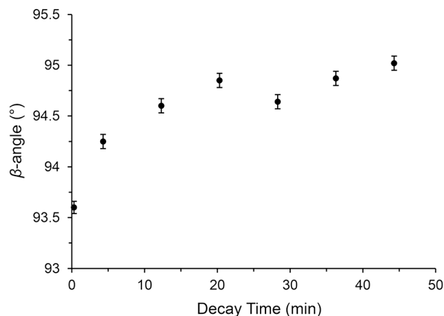
Fig. 7 SC-XRD kinetics experiments at 240 K, following the change in \beta -angle as a result of nitrite linkage isomerism. Top: Plot of \beta -angle vs. irradiation time under continuous illumination ( \lambda = 400 nm). Bottom: Plot of \beta -angle vs. decay time in the dark.
