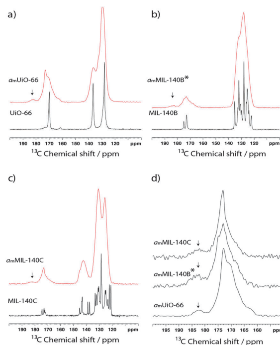
Fig. 3 ^{13}\text{C} MAS NMR spectra of crystalline (black) and amorphous (red) samples of (a) UiO-66 , (b) MIL-140B and (c) MIL-140C . (d) Magnified view of the 150\text{--}200 ppm region of the amorphous samples.
