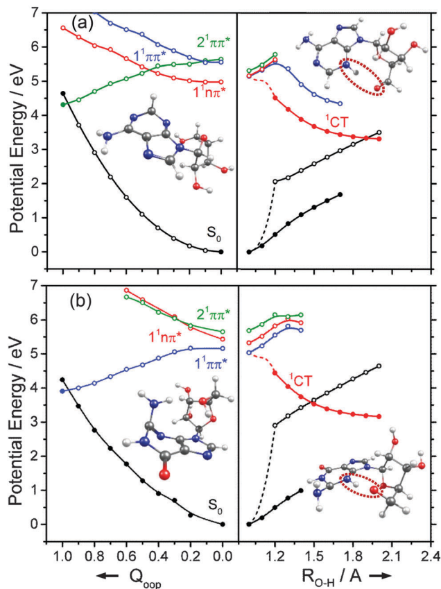
Fig. 15 Diabatic PECs for the ground and first three singlet excited states of (a) adenosine and (b) guanosine along Q_{\text{oop}} (left panel) and along the EDPT coordinate (right panel) calculated at CASPT2 and ADC(2) levels of theory, respectively. Filled points in the left hand panels represent the energies of the optimised critical structures ( i.e. the S_0 state minimum and the S_0/{}^1\pi\pi^* MECI – the optimised geometry of which is also shown). The convention for the use of open and filled points in the right hand panels is detailed in the text.
