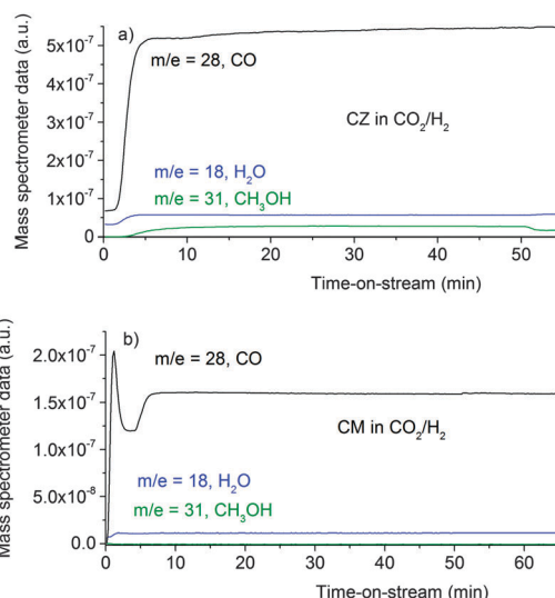
Fig. 4 Product analysis during methanol synthesis at 6.31 bar and 523 K over the CZ catalyst (a) and the CM catalyst (b) in CO 2 /H 2 feed gas (composition: 37.5 ml min -1 CO 2 , 150 ml min -1 H 2 and 1500 ml min -1 He).
