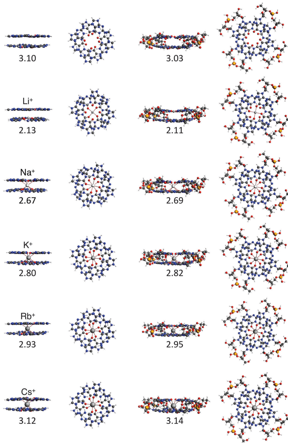
Fig. 4 Structures of \text{G}_4\text{-}[\text{ }]\text{-G}_4 , \text{G}_4\text{-M}^+\text{-G}_4 , GQ and \text{GQ-M}^+ where \text{M}^+ is an alkali metal cation (optimized at the ZORA-BLYP-D3(BJ)/TZ2P level of theory).
