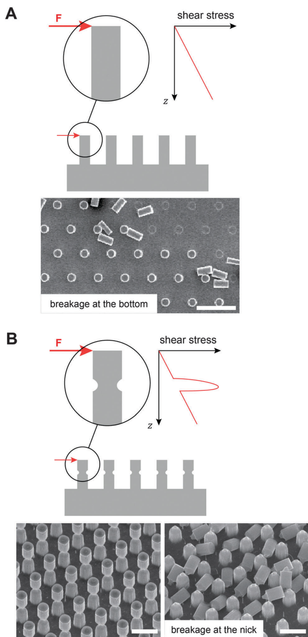
Fig. 17 Mechanical stability to resist shear loads, F , of submicron pillar structures. (A) Schematic illustration of increasing shear stress that has its maximum value at the substrate when the pillar has a constant cross-sectional area. Micrograph represents intact and pillars upon breakage. Scale bar: 20 \mu\text{m} . (B) Schematic illustration of a peak stress at the tapered, overhanging part of the pillar. Micrographs represent intact (left) and pillars upon breakage (right). Scale bars: 4 \mu\text{m} . Adapted from Hensel. 204
