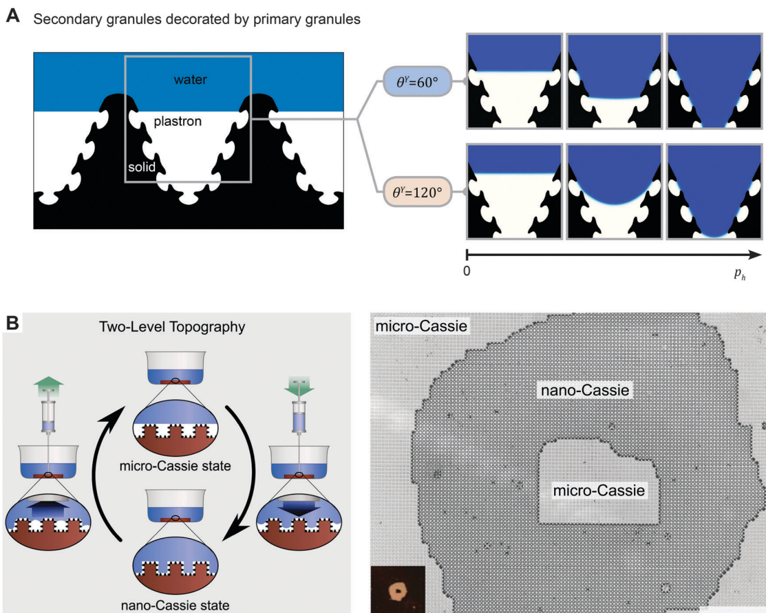
Fig. 16 Cassie–Wenzel transition on hierarchically assembled surfaces. (A) Numerical finite element method simulations showing the dynamics of the Cassie–Wenzel transition. On the left, a schematic representation of a sectional view of a hierarchically assembled surface, inspired by springtails. On the right, numerical results are presented by snap shots from left to right that display the advancing liquid front (blue) displacing the plastron (white) inside certain complex shaped solid phase fields (black). Both hydrophilic and hydrophobic surfaces were considered. (B) Wetting states and transitions on surfaces with two-level topography. Both the micro-Cassie and the nano-Cassie state can be visualized by optical microscopy upon complete immersion of the surface. (A) Adapted from Hensel et al. 105 under a Creative Commons Attribution 4.0. Full terms at http://www.creativecommons.org/licenses/by/4.0/ . (B) Reprinted with permission from Verho et al. 194
