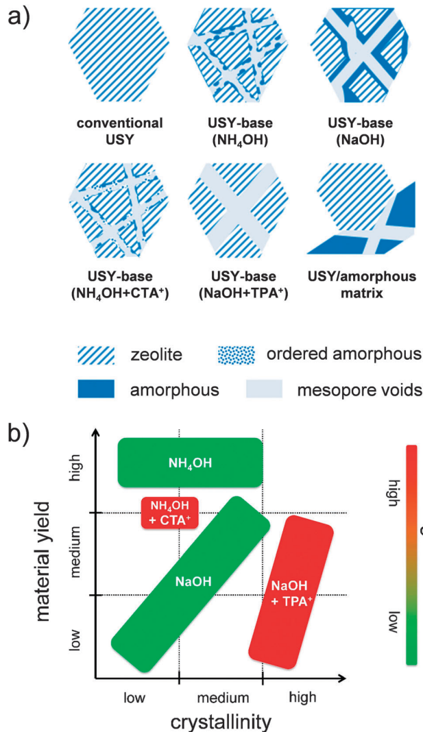
Fig. 10 (a) Overview of solids obtained by alkaline treatment of USY ( \text{Si}/\text{Al} > 15 ) using distinct approaches. 41 The use of \text{NH}_4\text{OH} and \text{NaOH} lead to (controlled) amorphisation and accordingly amorphous silica-alumina (ASA) zeolite composites. In the case of \text{NH}_4\text{OH} , the amount of solids leached is minimal. When \text{TPA}^+ is used in the alkaline solution, the crystallinity can be fully preserved during the alkaline treatment (see Fig. 1b). When \text{CTA}^+ is present during the alkaline treatment crystallinity is preserved to a lower extent compared to with \text{TPA}^+ , which can be attributed to the presence of MCM-41-type ordered amorphous materials (see Fig. 8). Although USY crystals can display reduced zeolite properties, the presence of well-localized intracrystalline mesopores render them superior catalyst compared to mechanical mixtures of USY/ASA, which feature similar bulk crystallinity and porosity. (b) Plot highlighting the relation between the material yield, crystallinity, and used organics. 41 Thus far, the synthesis of highly-crystalline hierarchical USY zeolites can only be attained using organics such as DEA or \text{TPA}^+ . On the other hand, highly mesoporous samples with high solid yield are attained using \text{NH}_4\text{OH} treatment. Reprinted with permission from Wiley-VCH Verlag.
