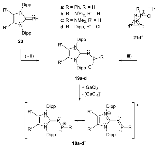
Scheme 7 Two different approaches for the synthesis of NHC stabilized chlorodiphosphenes 19a-d comprising bonding motif B. For 19a,b : (i) +R_2PCl_2, +DABCO, -DABCO\cdot HCl ; for 19c : (ii) +2PCl(NMe_2)_2, +DABCO, -DABCO\cdot HCl, -P(NMe_2)_3 ; for 19d : (iii) +3 1,3-bis(2,6-diisopropylphenyl)-4,5-dichloro-imidazole-2-ylidene, 5 + . Subsequent chloride abstraction yields polarized cationic diphosphenes 18a-d + . Only two resonance structures that indicate the polarization of 18a-d + are shown.
