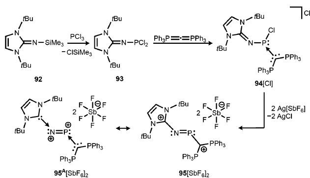
Scheme 22 Reaction of imino phosphorus dichloride to the phosphonium salt 94 [Cl] and its conversion to the dicationic phosphiminine 95 2+ . Phosphorus mononitride formulation 95 A2+ .
