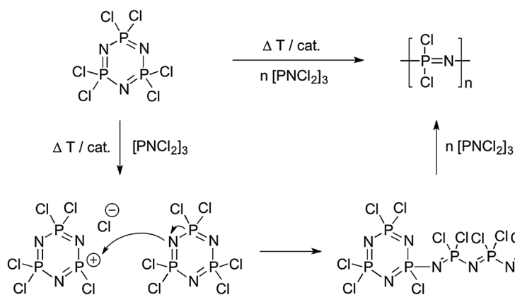
Fig. 5 Thermally and/or catalytically induced ring opening polymerisation representing the classical route to synthesise poly(dichloro)phosphazene [\text{NP}(\text{Cl}_2)_2]_n and its commonly accepted mechanism.
