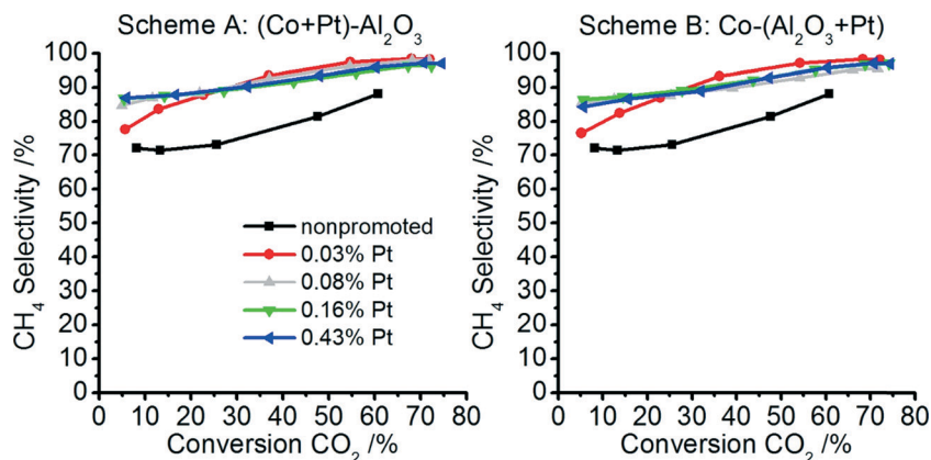
Fig. 10 \text{CH}_4 selectivities at different \text{CO}_2 conversions for the non-promoted \text{Co}-\text{Al}_2\text{O}_3 catalyst and for the platinum-promoted catalysts prepared according to preparation scheme A (tight contact of Pt and Co) and scheme B (tight contact of Pt and Al).
