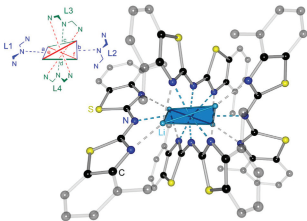
Fig. 8 Molecular structure of [\text{Li}(\text{4-MeNCSC}_6\text{H}_3)_2\text{N}]_4 ( 8 ). To clarify the binding motif co-crystallised solvent molecules and hydrogen atoms are omitted as well as the annulated moieties are represented in faded colour. In the upper left corner a simplified model of the coordination environment is depicted.
