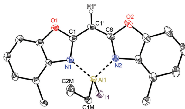
Fig. 9 Molecular structure of [\text{IEtAl}\{(\text{4-MeNCOC}_6\text{H}_3)_2 \text{CH}\}] (7). Anisotropic displacement parameters are depicted at the 50% probability level. C–H hydrogen atoms are omitted for clarity except for the one at the bridging CH group. Structural data are given in Tables 1–3.
