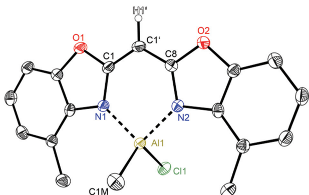
Fig. 7 Molecular structure of [\text{ClMeAl}\{(\text{4-MeNCOC}_6\text{H}_3)_2 \text{CH}\}] (5). Anisotropic displacement parameters are depicted at the 50% probability level. C–H hydrogen atoms are omitted for clarity except for the one at the bridging CH group. Structural data are given in Tables 1–3.
